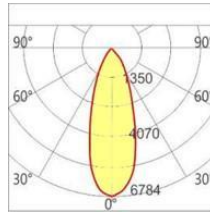
GEFEST36 LED
