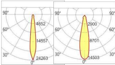
GEFEST15 LED
